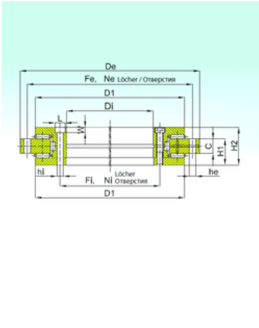
YRT 395 Bearing 2D drawings and 3D CAD models
