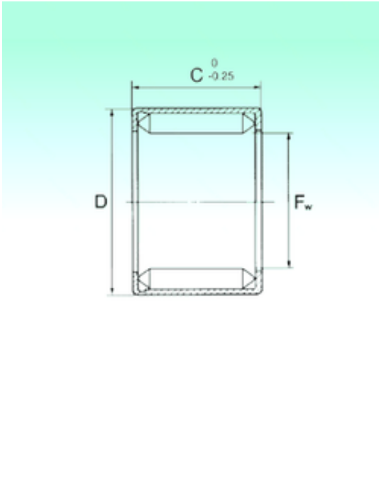
HN1212 Bearing 2D drawings and 3D CAD models
