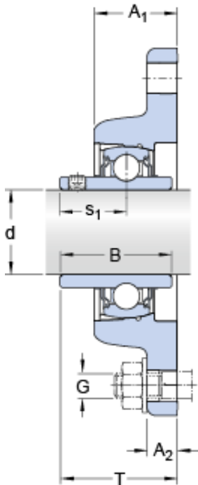
FYT 1.1/2 TF/VA228 Bearing 2D drawings and 3D CAD models
